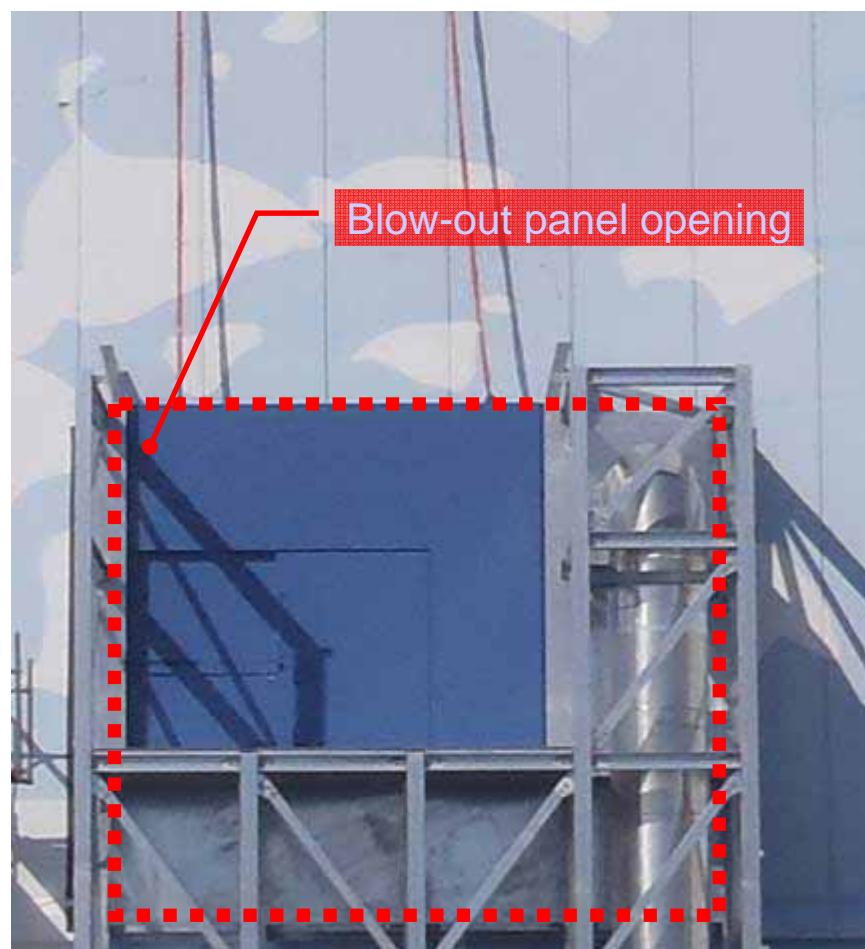
Closure panel installation completed
