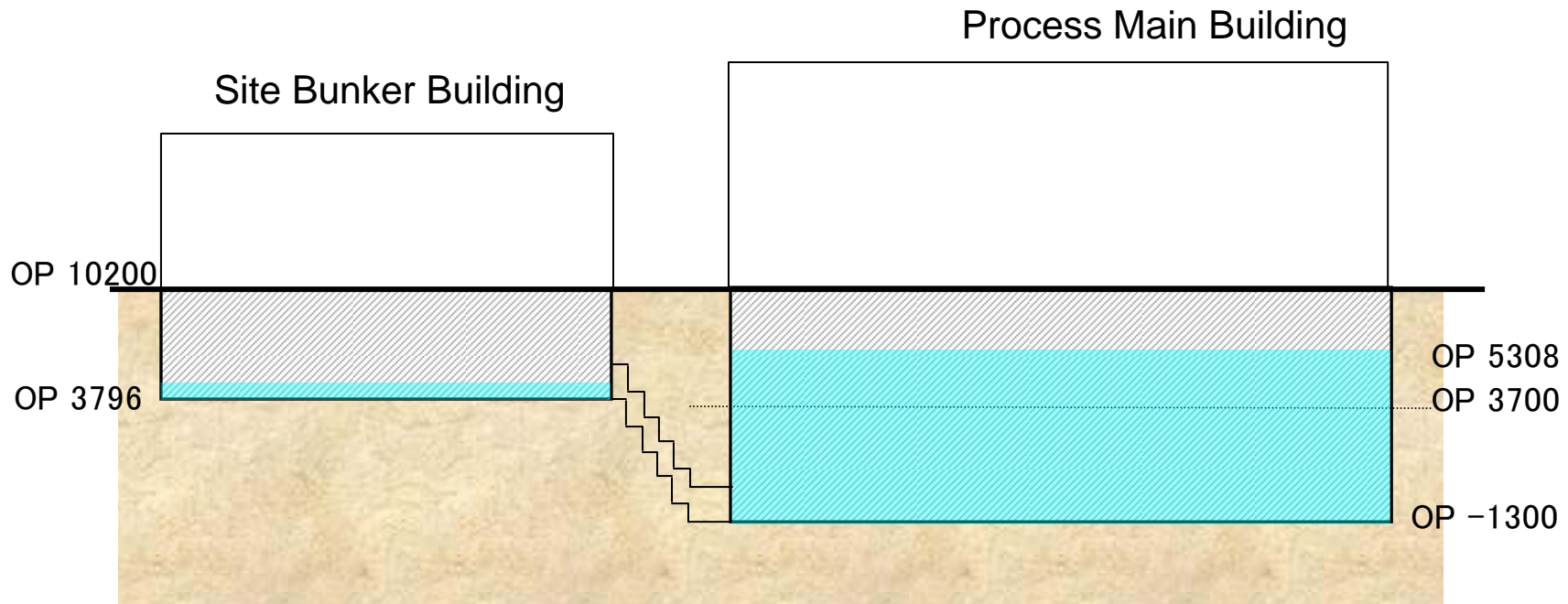
Cross-section diagram of site bunker
