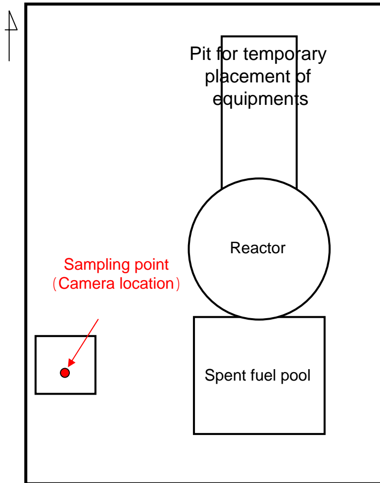
Layout of 5 th floor in reactor building (Unit 3, Fukushima Daiichi Nuclear Power Station)
