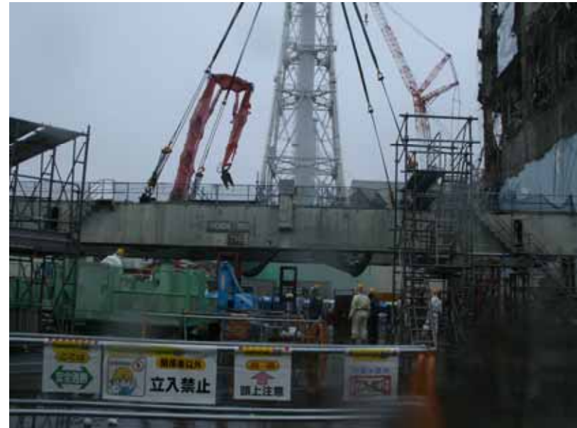
Removal works of the girder of overhead traveling crane (4) March 5, 2012
