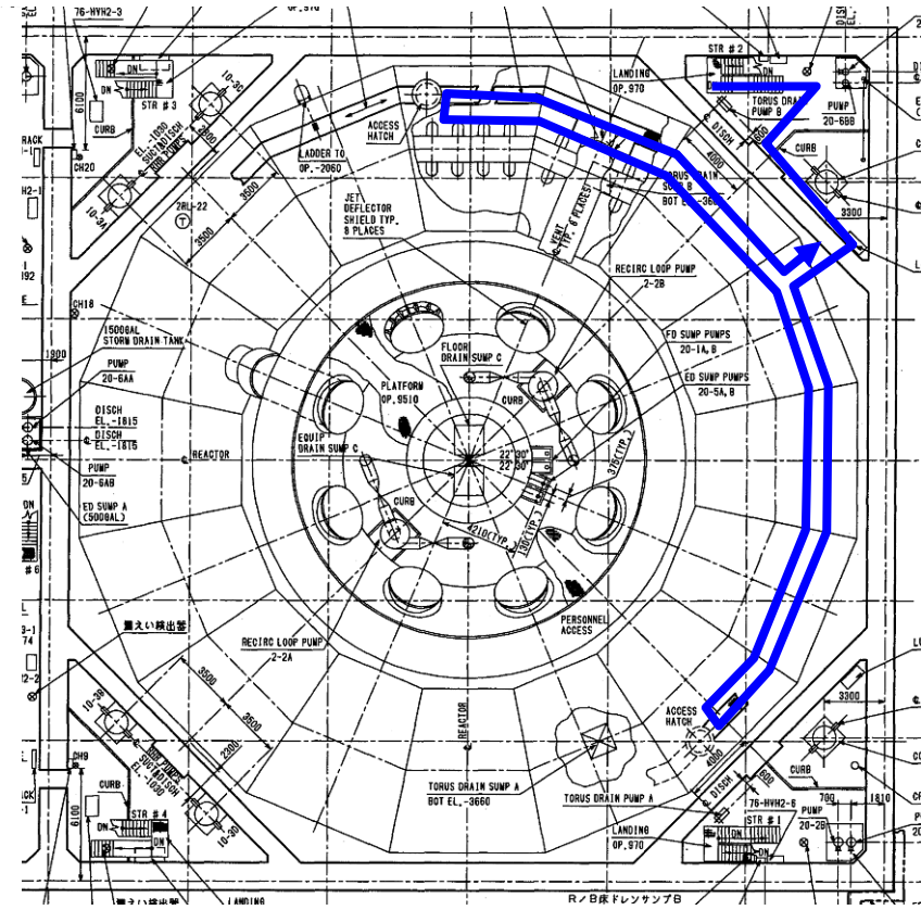
Reactor Building, B1
