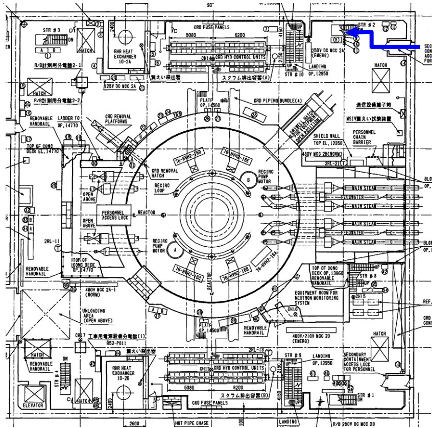
Reactor Building, 1F
