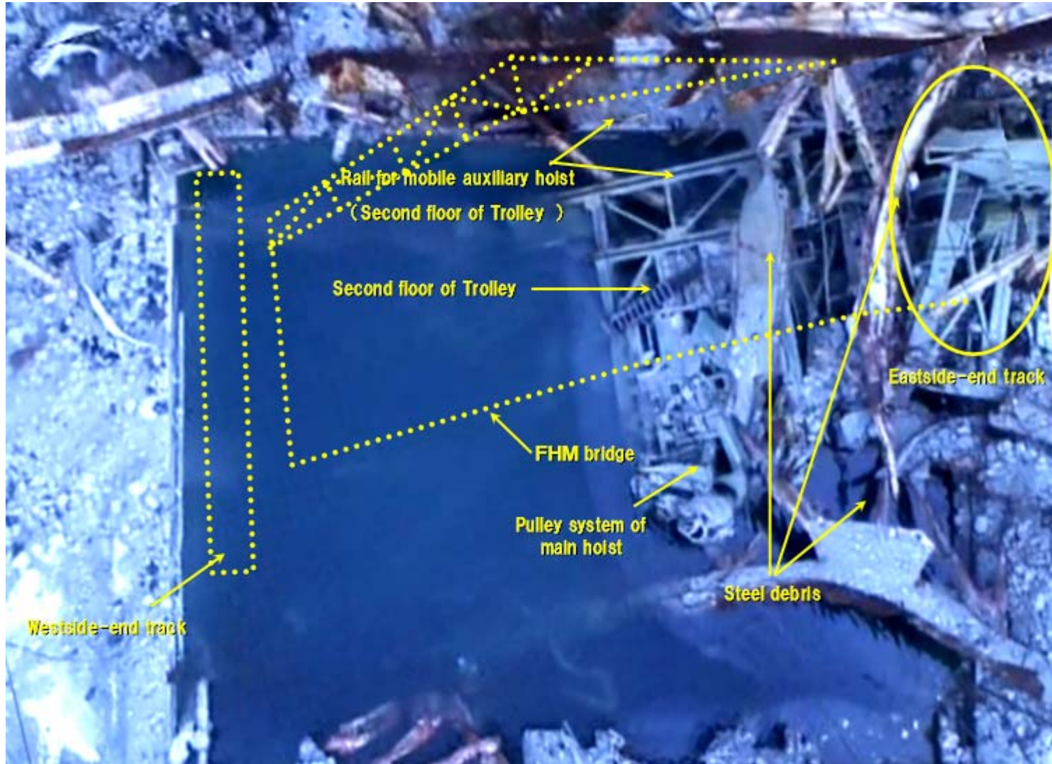
Presumption of Refueling machine's situation (October 15)
