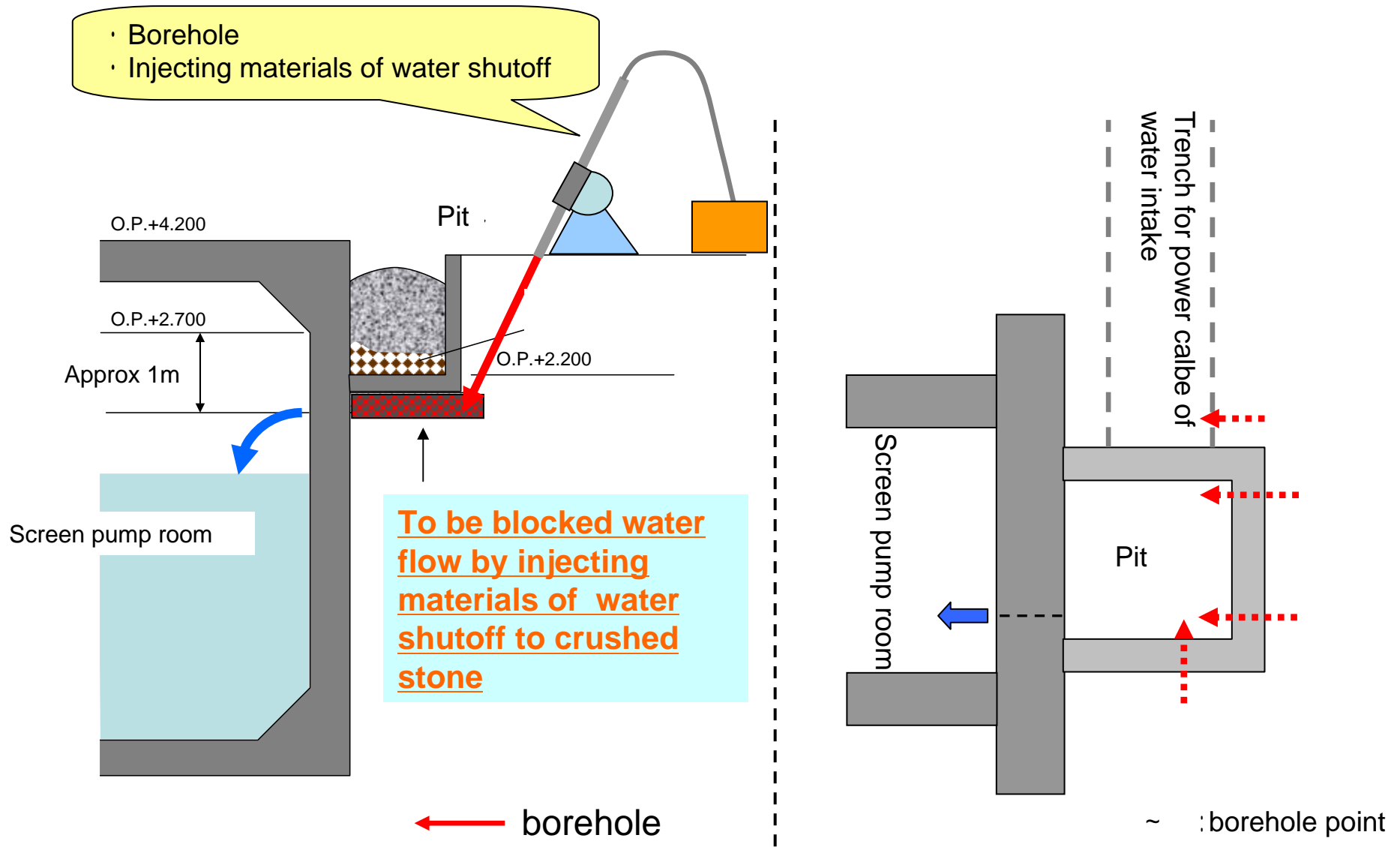
A-A Section view
