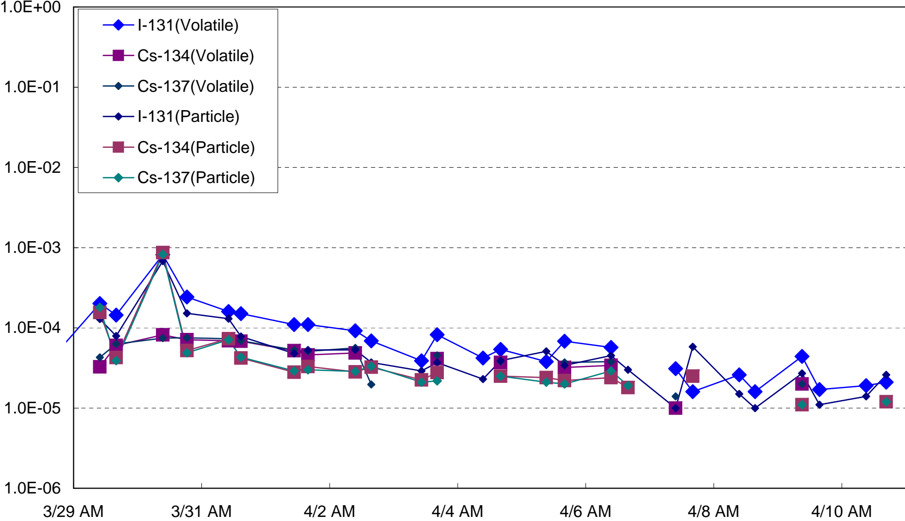
Fukushima Daini: the result of the dust nuclide analysis
