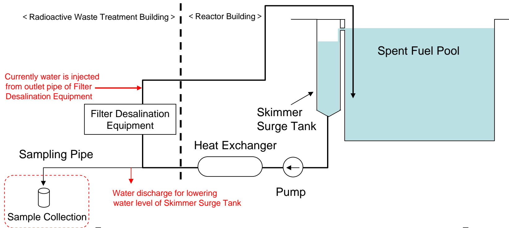
【 Spent Fuel Pool Cooling and Purification System 】
