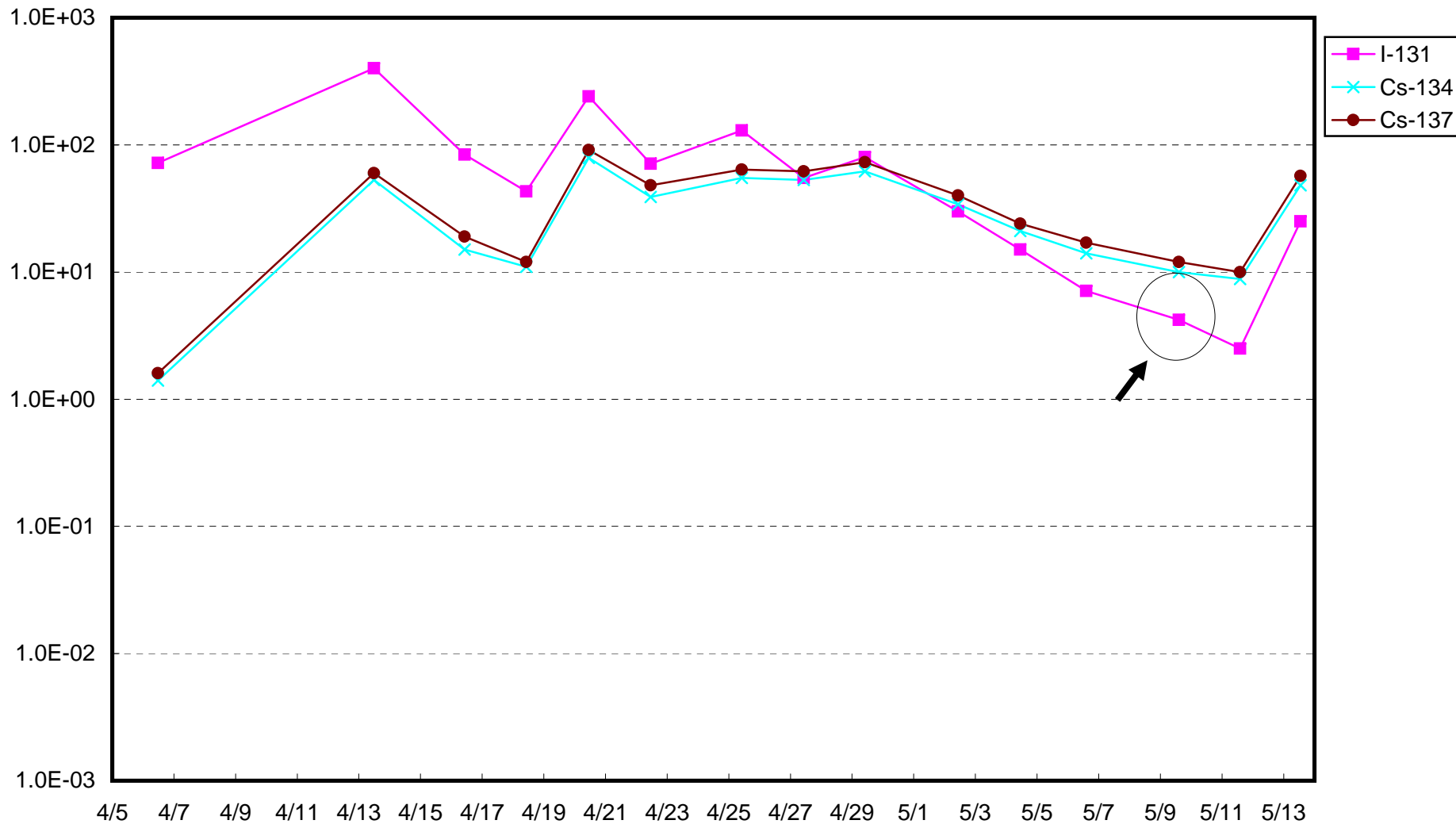
Fukushima Daiichi Nuclear Power Station: Radioactivity Density of Sub-drain at Unit 1 (Bq/cm 3 )
