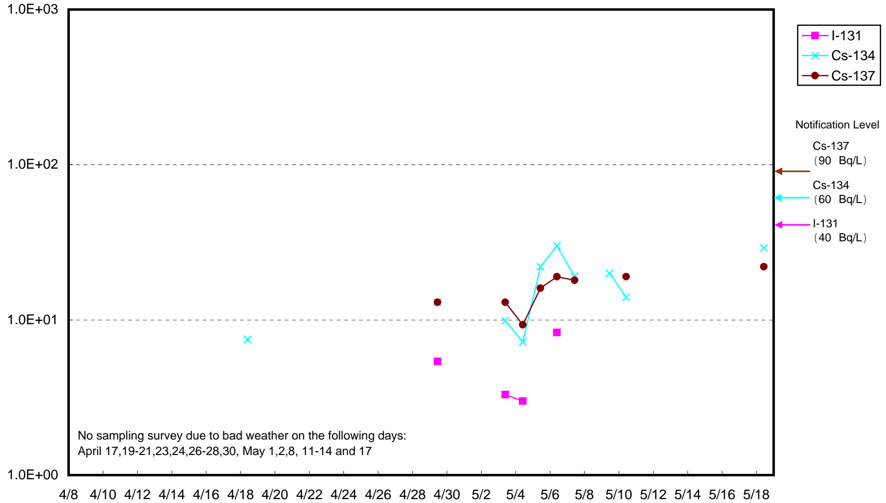
Radioactivity Density of Seawater around 3 km offshore of Haramachi-ku (Bq/L) (Upper layer)
