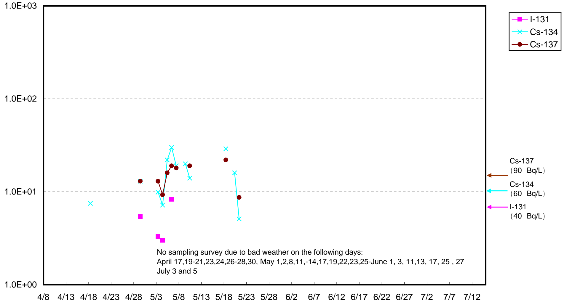
Radioactivity Density of Seawater around approx. 3km offshore of Haramachi district Upper Layer (Bq/L)
