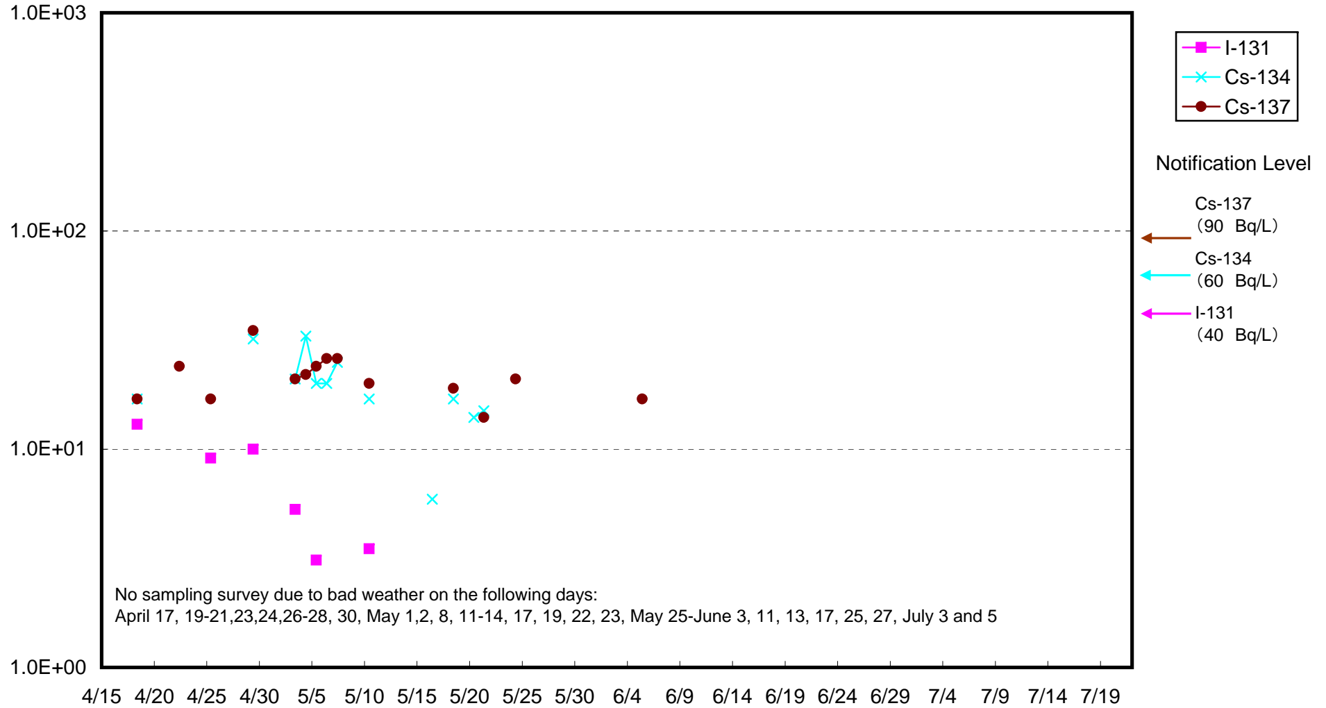
Radioactivity Density of Seawater around approx. 8km offshore of Odaka Area Upper Layer(Bq/L)
