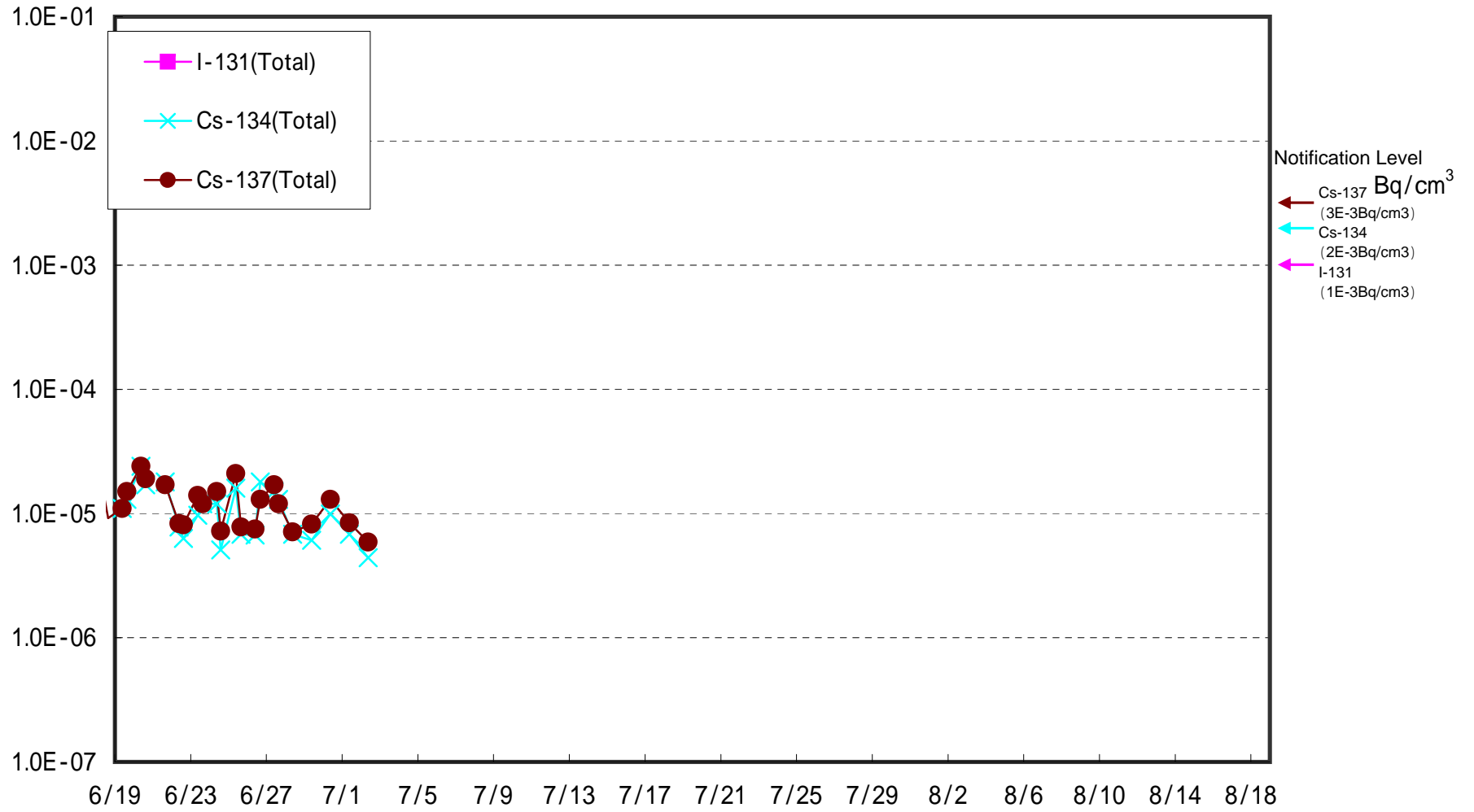
MP-1 (Reference) Fukushima Daini Nuclear PowerStation Results of Dust Nuclide Analysis (Bq/cm 3 )
