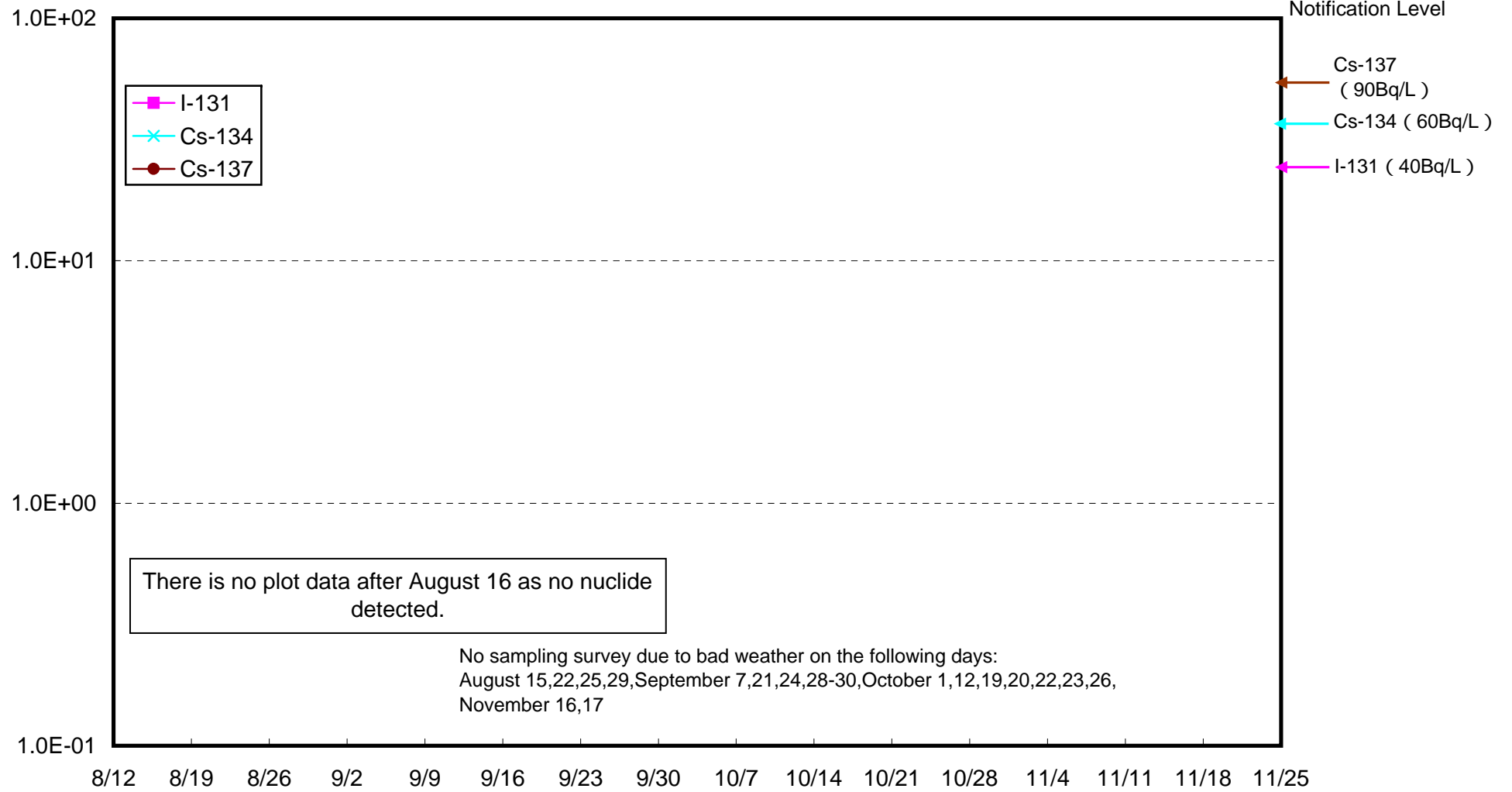
Radioactivity Density of Seawater 15km Offshore of Minami Soma-shi Shore Upper Layer (Bq/L)
