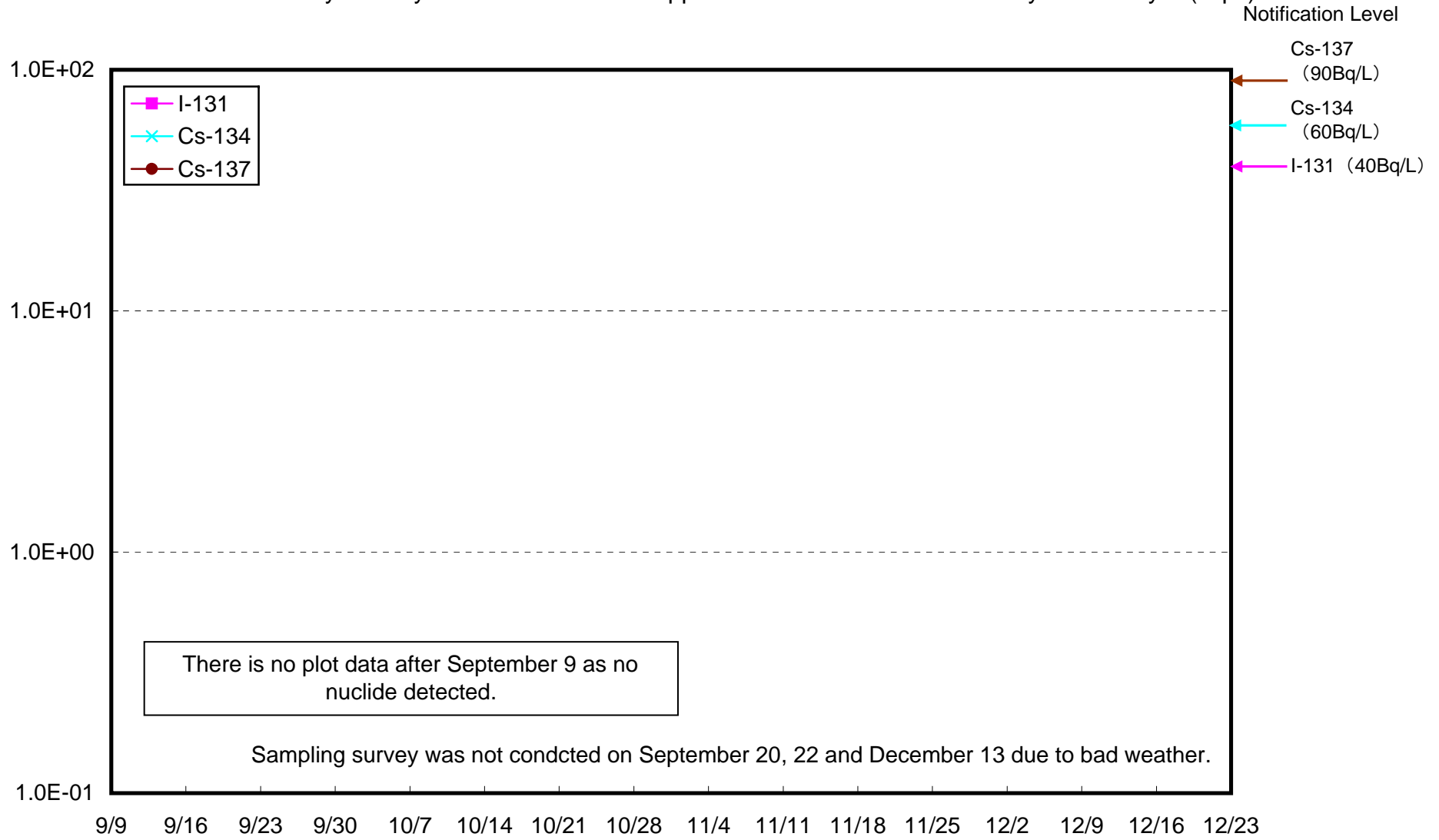
Radioactivity Density of Seawater around approx. 3 km offshore of Soma City Lower Layer (Bq/L)
