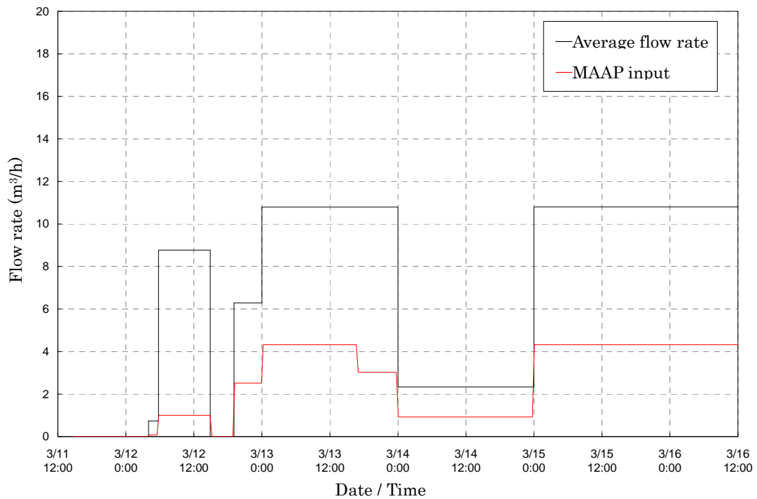
Figure 1 Amount of water injection assumed in MAAP analysis for Unit-1*1
