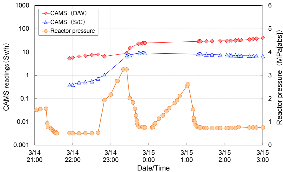
Figure 12 CAMS readings and reactor pressure
