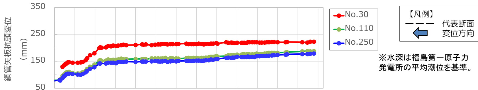
[杭頭変位の経時変化]
